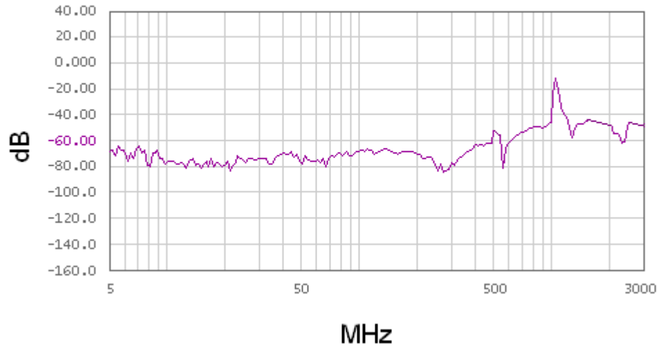
Forward to MoCA Path Isolation
