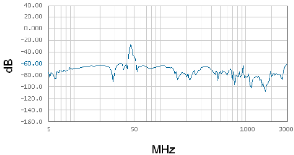
Reverse to Forward Path Isolation
