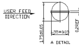
A DETAIL
